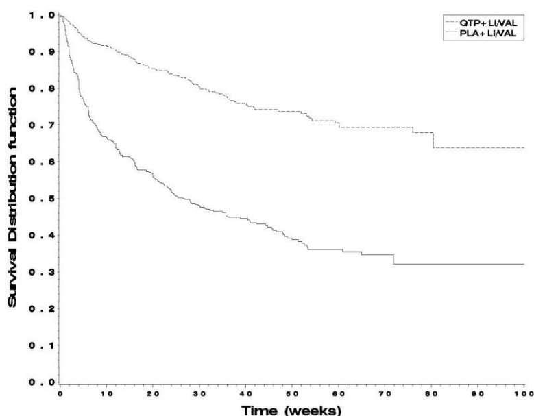
Figure 1 Time to recurrences of a mood event for the combined maintenance treatment studies, Kaplan Meier curves (ITT population)
