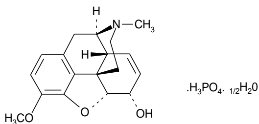
Codeine phosphate hemihydrate
