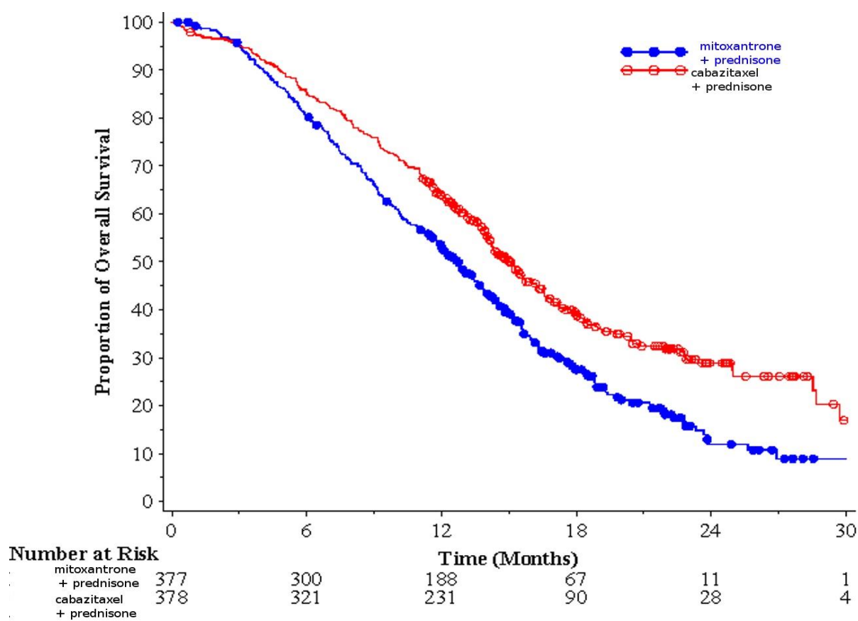
Figure 1 - Kaplan-Meier Overall Survival Curves (EFC6193)
