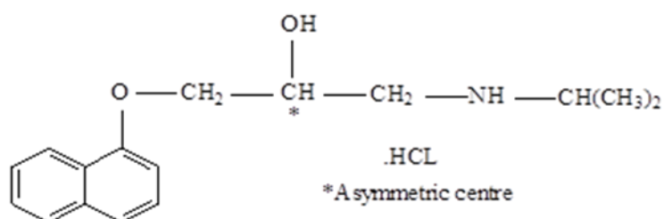
Figure 1 Chemical structure of propranolol hydrochloride
