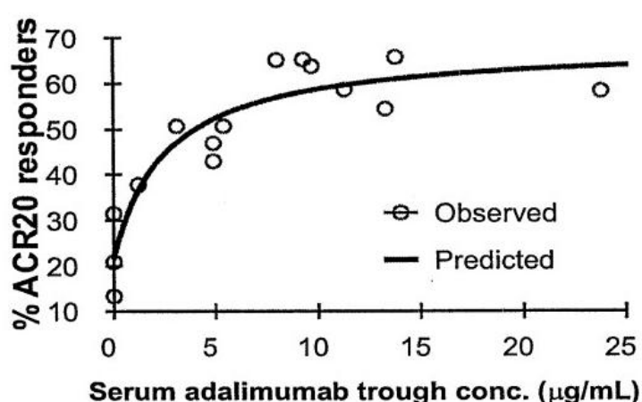
Figure 1: Concentration-Efficacy Relationship
